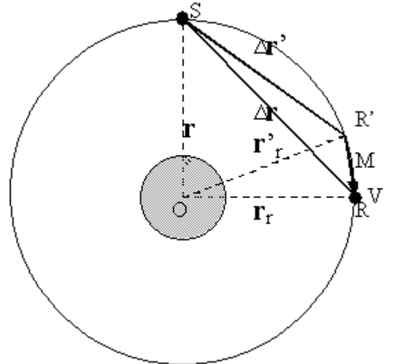
Fig. 8 The Sagnac correction for using the position of the second satellite at the transmission time
