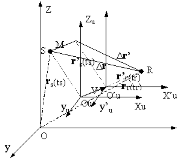
Fig. 9 The Sagnac correction in system U
