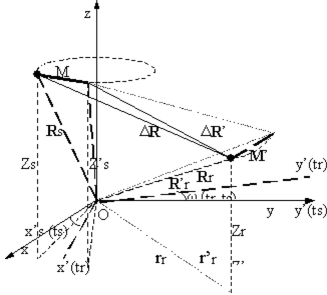
Fig.7 The Sagnac correction in ECEF
